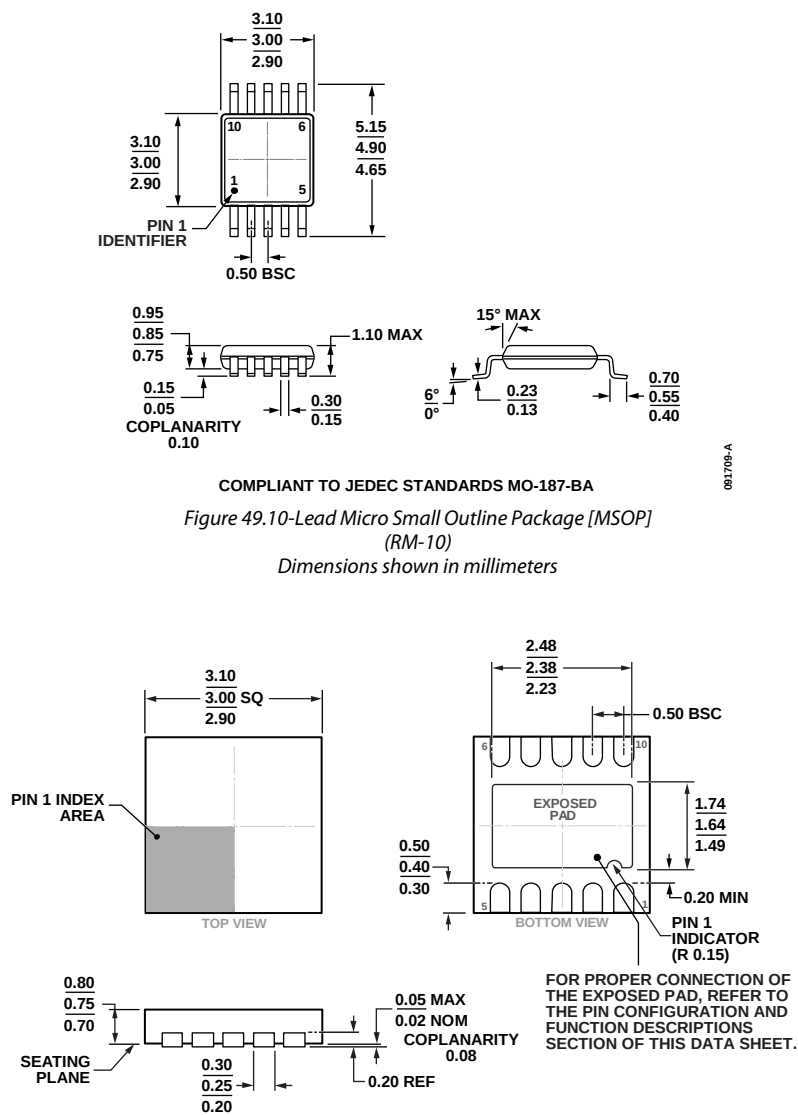
Figure 50. 10-Lead Lead Frame Chip Scale Package [LFCSP_WD] 3 mm x 3 mm Body, Very Very Thin, Dual Lead (CP-10-9) Dimensions shown in millimeters
