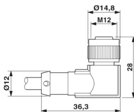
Socket M12 x 1, angled, with LED
