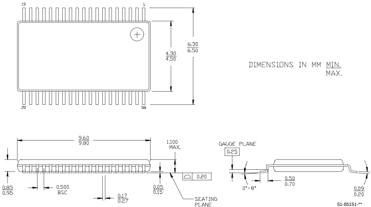
38-lead TSSOP (4.40 mm Body) Z38
