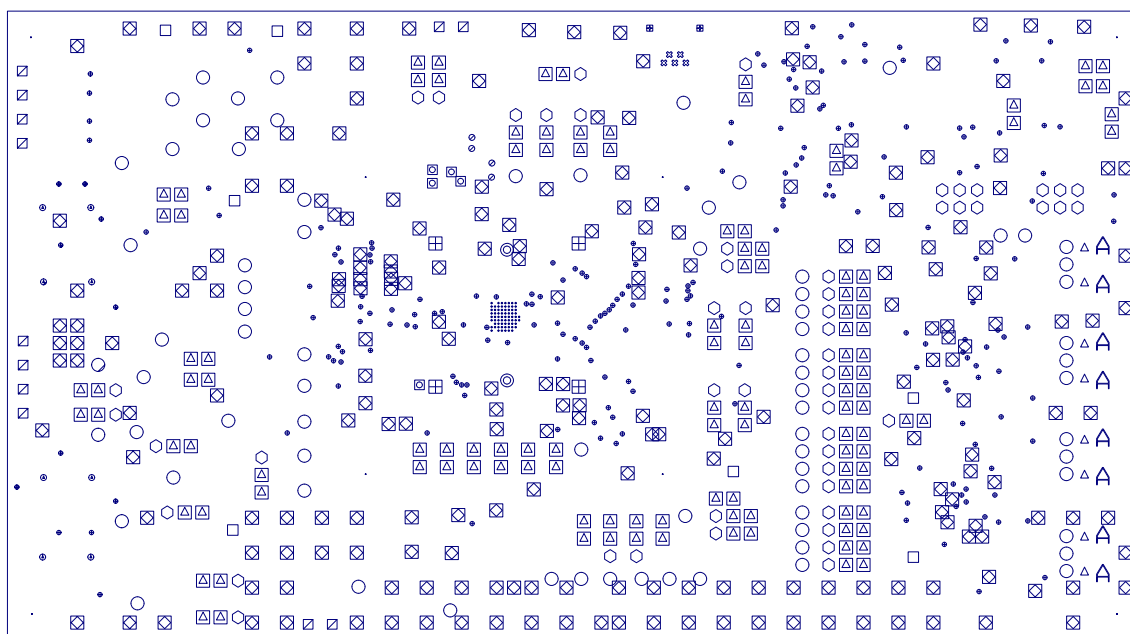
Figure 14. TLV320AIC3262EVM PCB Drill Pattern
