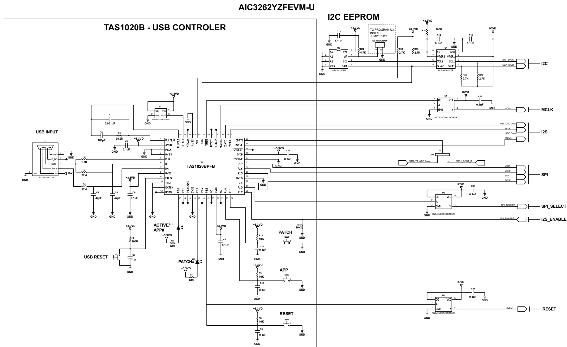
Figure 16. Schematic, Sheet 2 of 6
