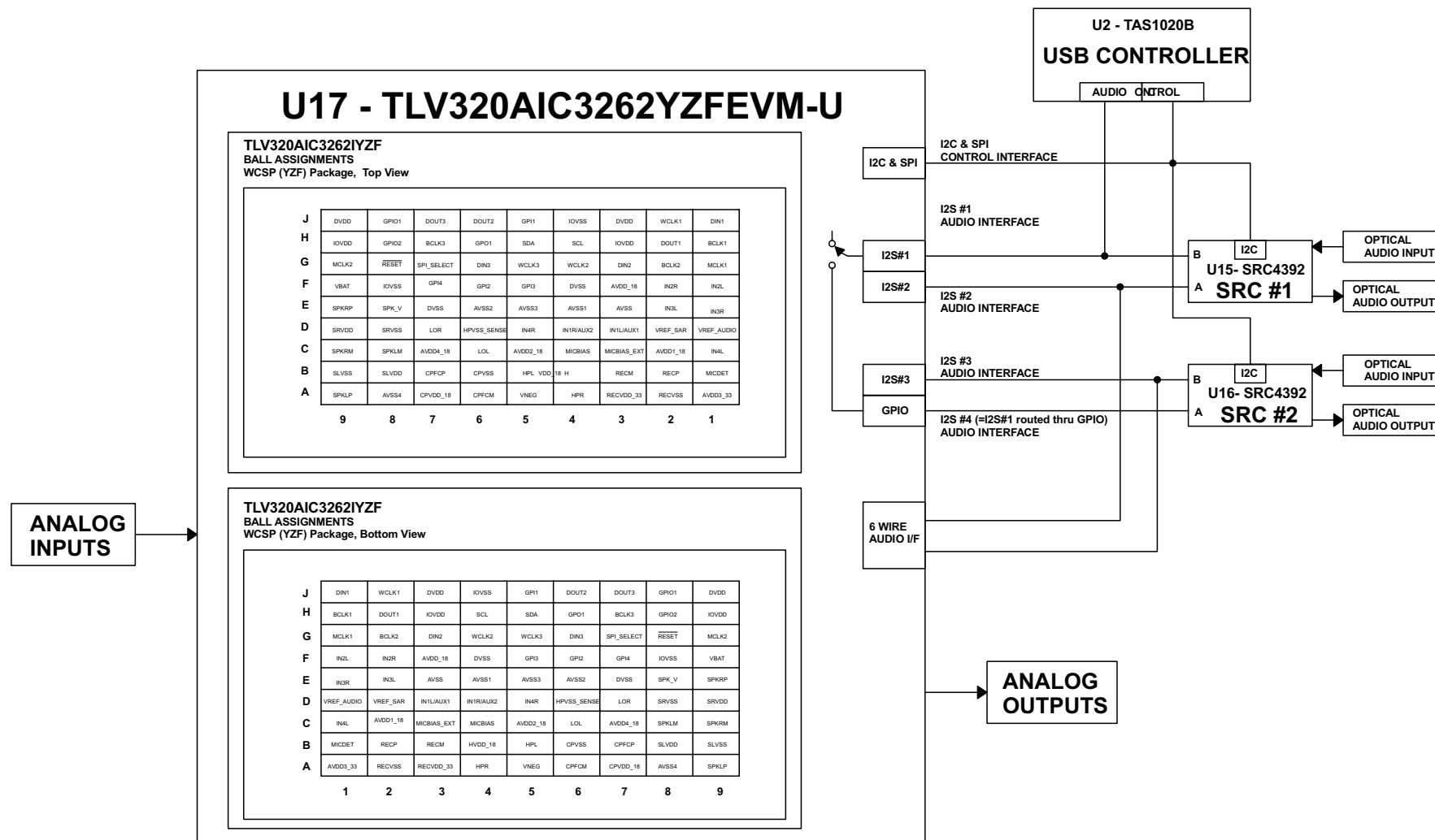
Figure 15. Schematic, Sheet 1 of 8
