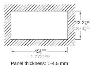
Panel cutout dimensions
