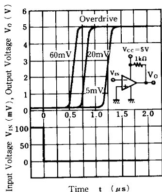
Transfer Characteristics (1)
