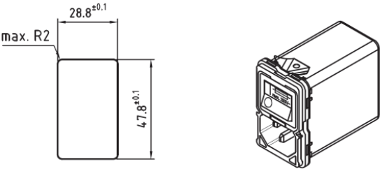
Panel cutout:
