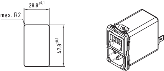
Panel cutout:
