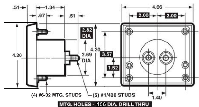
4-1/2" Models 2124, 2124T, 2144, 2154, 2184
