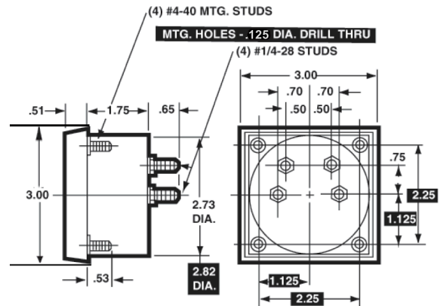
3-1/2" Model 2173
