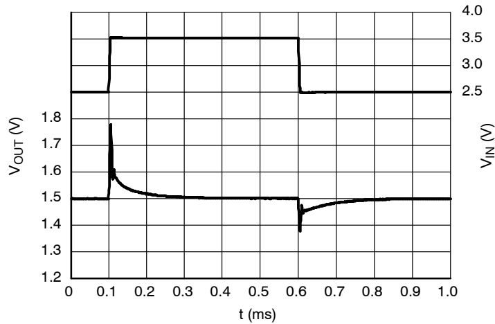
Figure 23. Line Transients, 1.5 V Version, t_R = t_F = 5 \mu s , I_{OUT} = 30 mA
