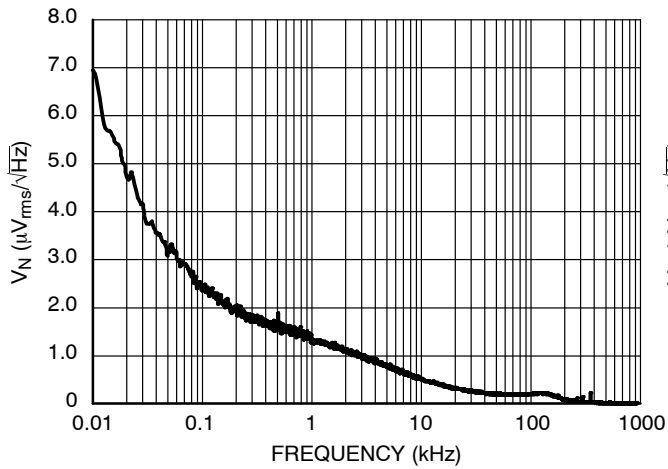
Figure 21. Output Voltage Noise, 2.5 V Version, V_{IN} = 3.5 V , I_{OUT} = 30 mA
