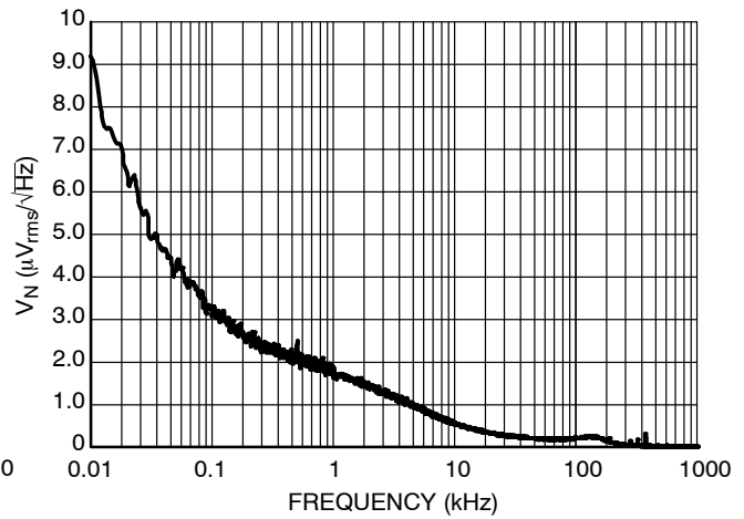
Figure 22. Output Voltage Noise, 3.3 V Version, V_{IN} = 4.3 V , I_{OUT} = 30 mA
