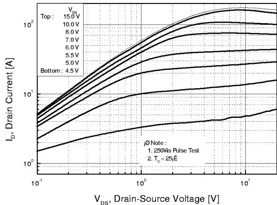
Fig 1. Output Characteristics
