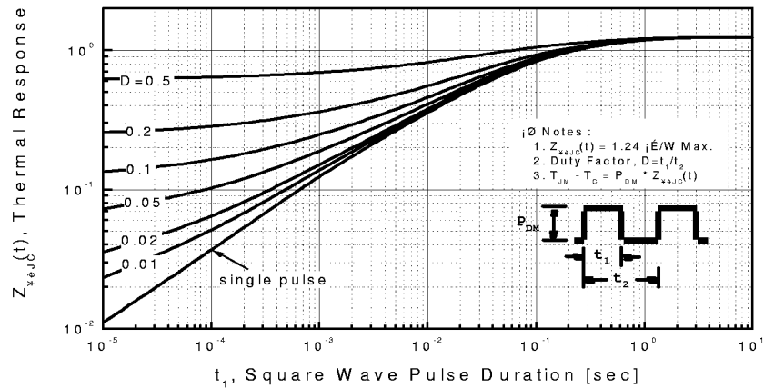
Fig 11. Thermal Response
