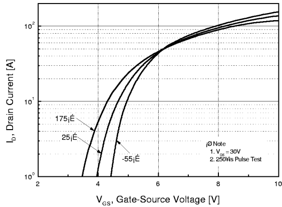
Fig 2. Transfer Characteristics
