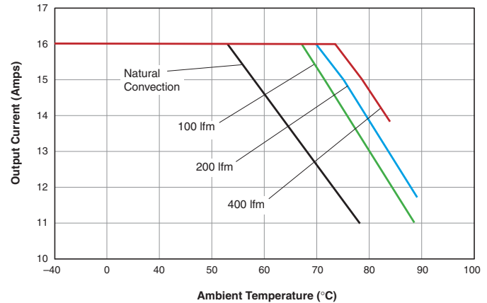
LSN-2.5/16-D12 Output Current vs. Ambient Temperature (Vertical mount, air flow direction from input pins to output pins)
