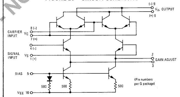
FIGURE 23 — CIRCUIT SCHEMATIC
