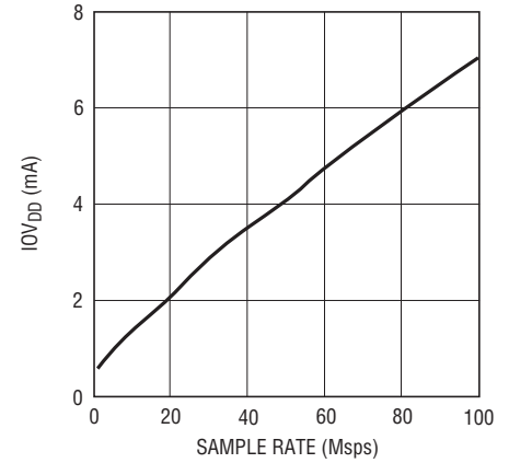
LTC2223: I_{OVDD} vs Sample Rate, 5MHz Sine Wave Input, -1\text{dB} , 0V_{DD} = 1.8V
