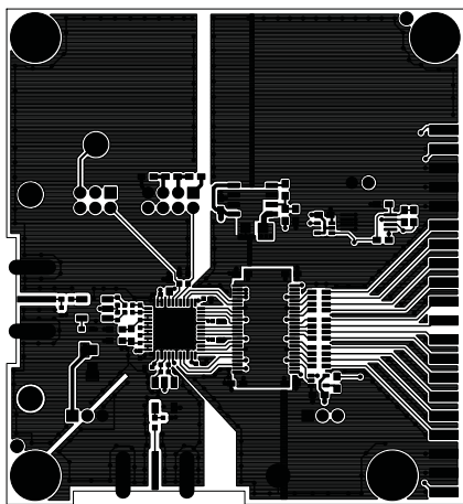
Layer 1 Component Side
