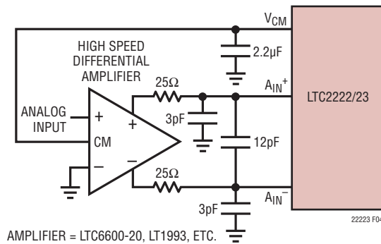
Figure 4. Differential Drive with an Amplifier
