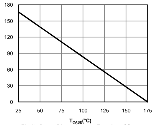
Fig 10: Power Dissipation as a Function of Case
