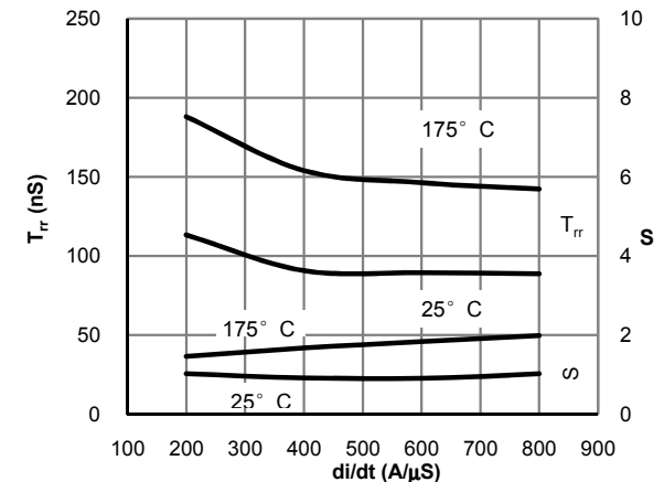
Fig 24: Diode Reverse Recovery Time and Softness Factor vs. di/dt ( V_{GE}=15V, V_{CE}=400V, I_F=10A )
