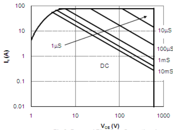
Fig 9: Forward Bias Safe Operating Area ( T_C=25^\circ\text{C} , V_{GS}=15\text{V} )
