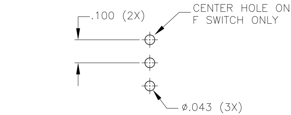
RECOMMENDED PCB LAYOUT TOLERANCES +/- .002
