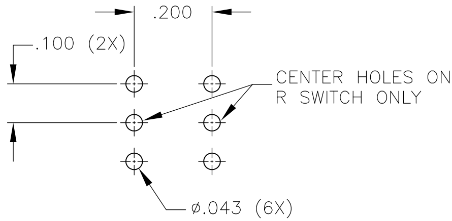
RECOMMENDED PCB LAYOUT TOLERANCES +/- .002
