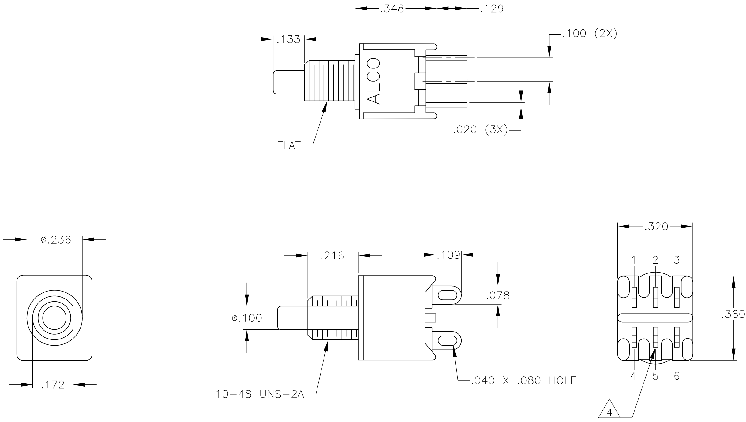
TPC23M, TPC23R
