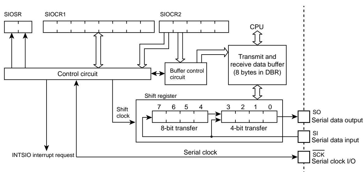
Figure 14-1 Serial Interface
