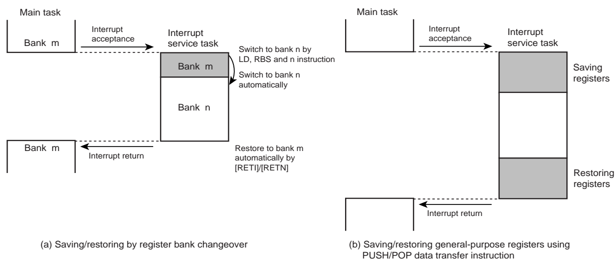
Figure 3-4 Saving/Restoring General-purpose Registers under Interrupt Processing
