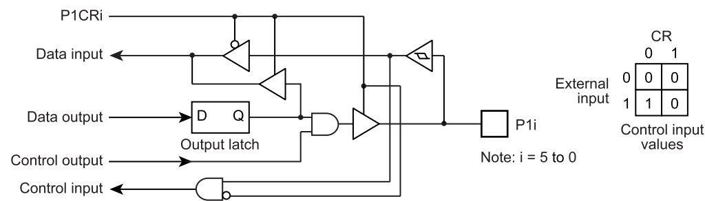
Figure 5-2 Port P1
