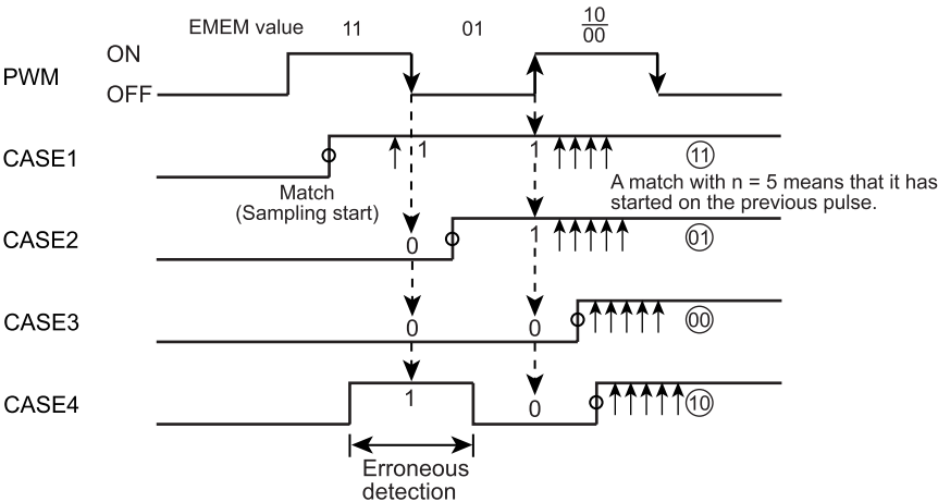
Figure 12-6 Detection Timing of the Position Detection Position
