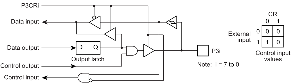
Figure 5-4 Port P3
