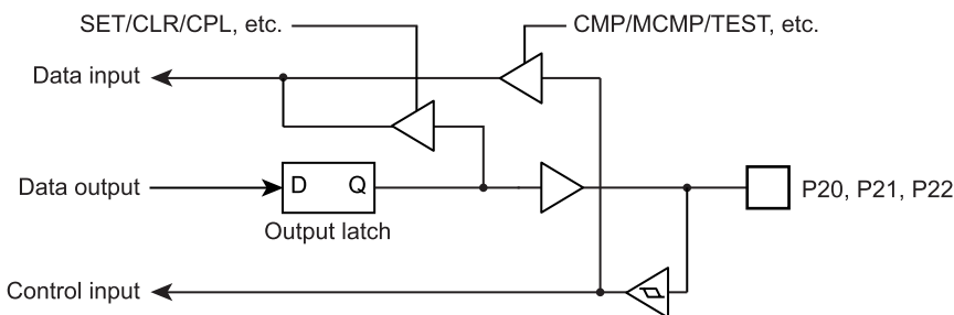
Figure 5-3 Port P2
