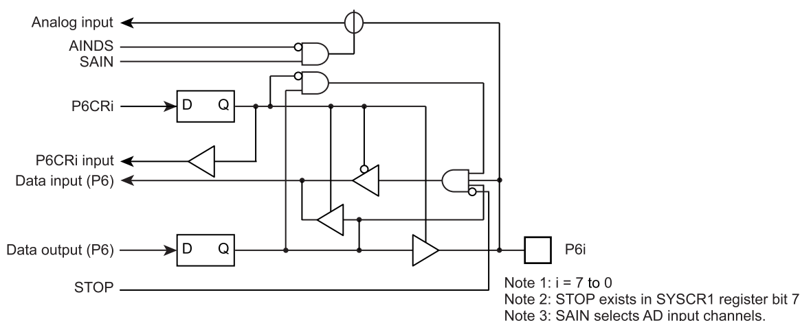
Figure 5-6 Port P6
