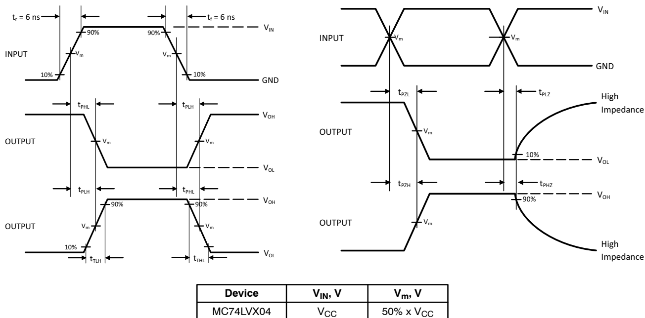
Figure 3. Switching Waveforms
