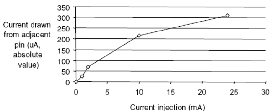
Figure 174. Impact of negative current injection on adjacent pin
