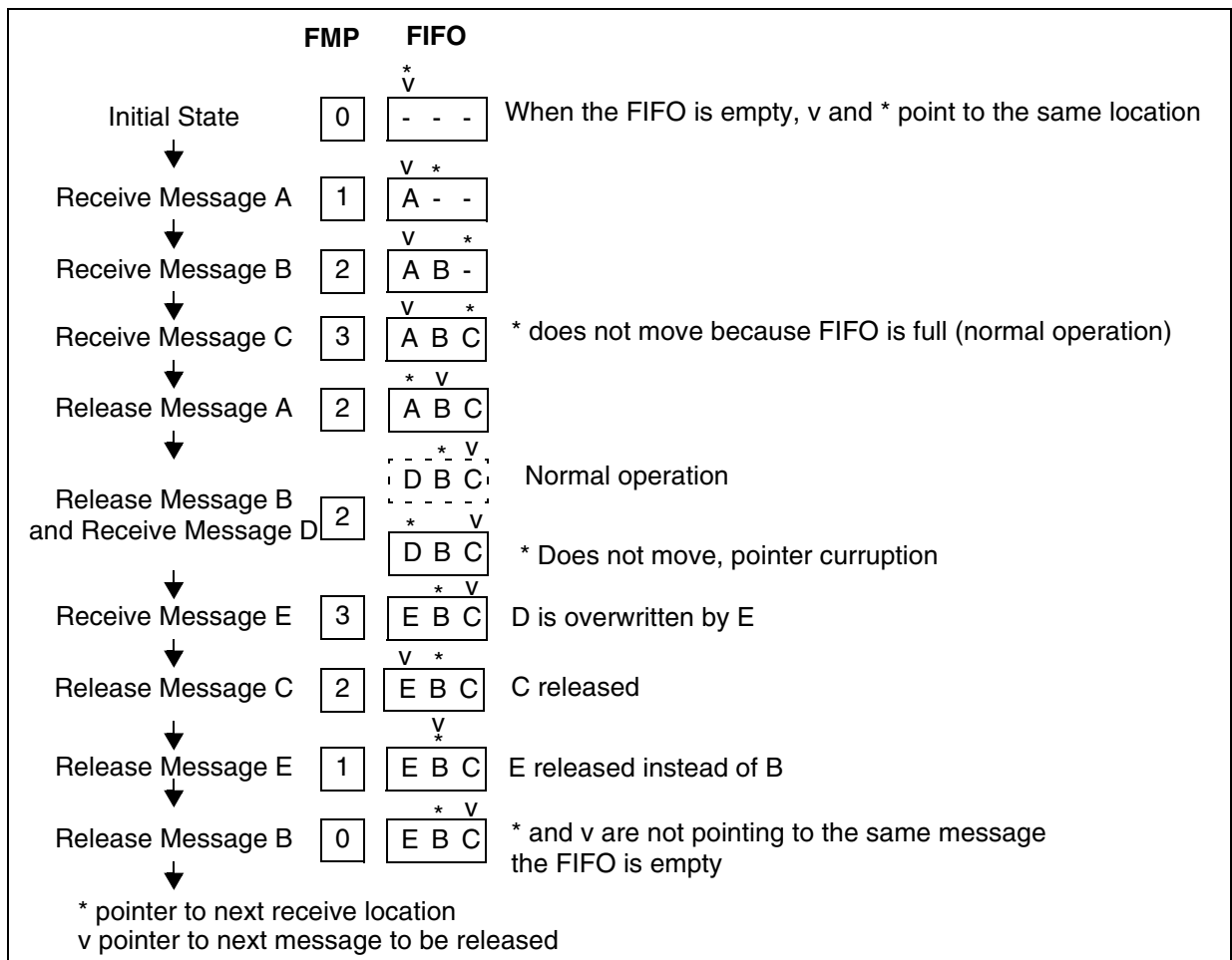
Figure 168. FIFO Corruption
