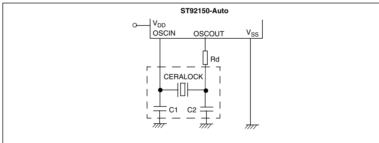
Figure 69. Test Circuit
