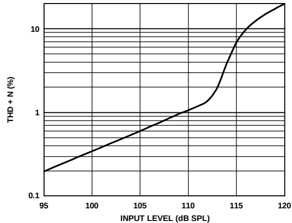
Figure 7. THD+N vs. Input SPL
