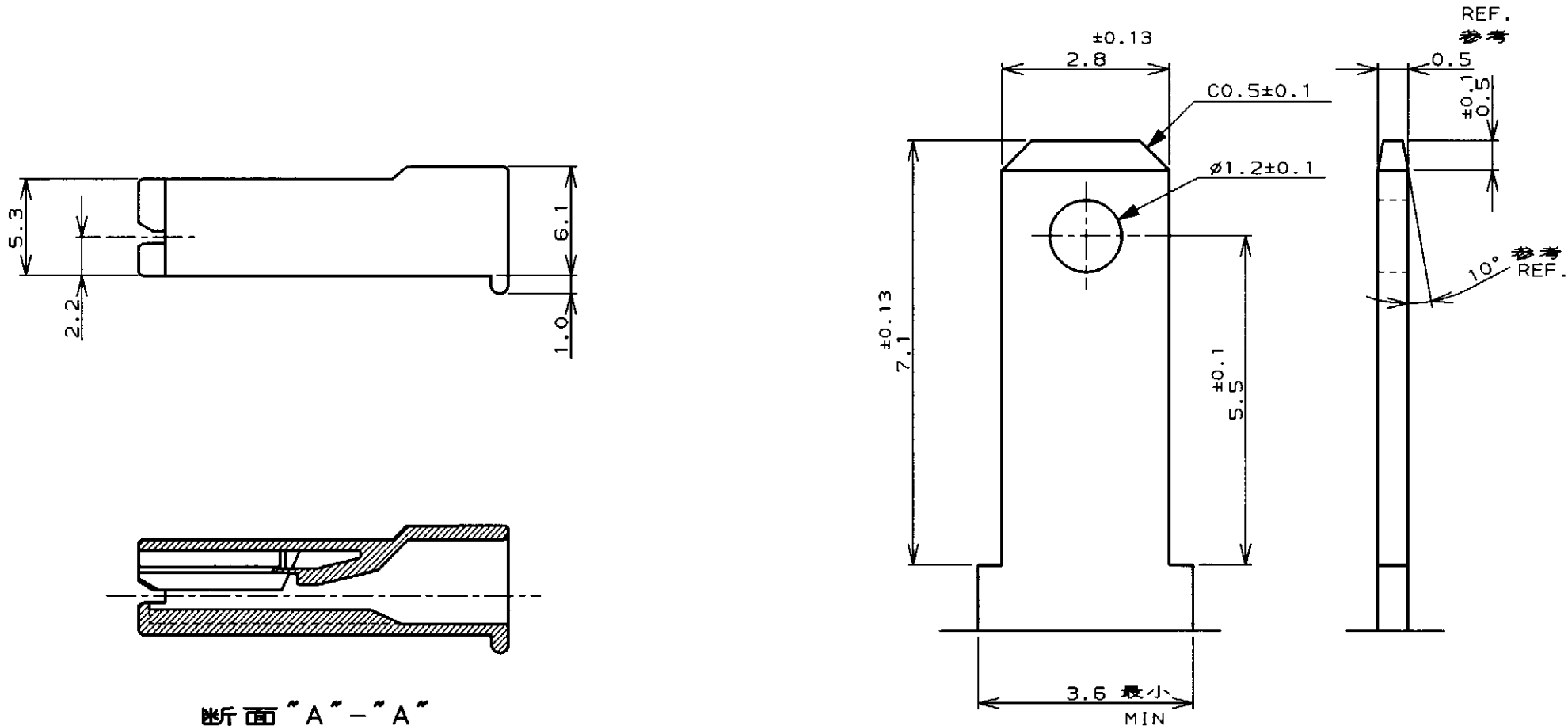
推奨タブ図 APPLICABLE TAB DIMENSIONS
