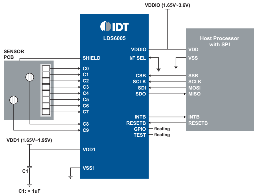
Figure 2. LDS6005 application diagram
