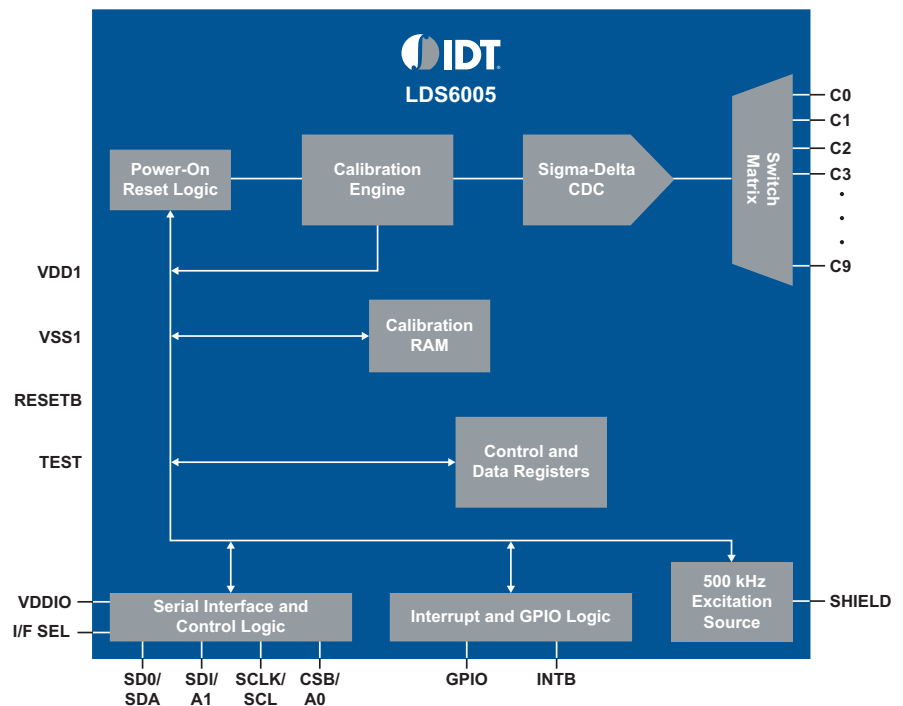
Figure 1. LDS6005 block diagram
