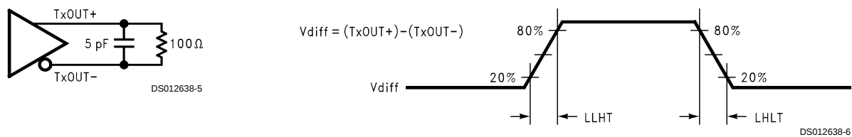
FIGURE 2. DS90CR281 (Transmitter) LVDS Output Load and Transition Timing
