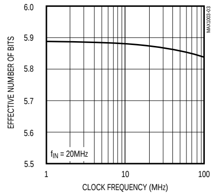
EFFECTIVE NUMBER OF BITS vs. SAMPLING/CLOCK FREQUENCY
