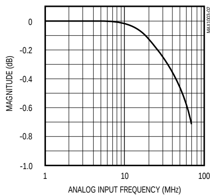
ANALOG INPUT BANDWIDTH
