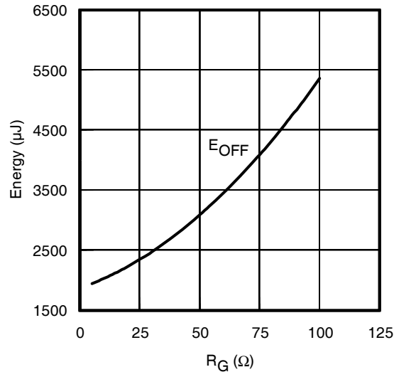
Fig. 15 - Typ. Energy Loss vs. R_G T_J = 150^\circ\text{C} ; L = 200\mu\text{H} ; V_{CE} = 600\text{V} ; I_{CE} = 30\text{A} ; V_{GE} = 15\text{V}
