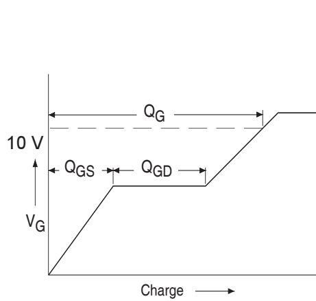
Fig 12a. Basic Gate Charge Waveform
