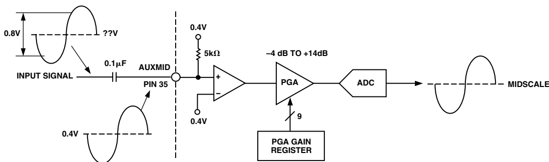
Figure 6. AUXMID-Mode Circuit Block Diagram
