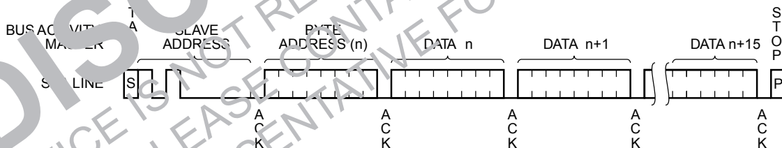
Figure 9: Page Write Timing
