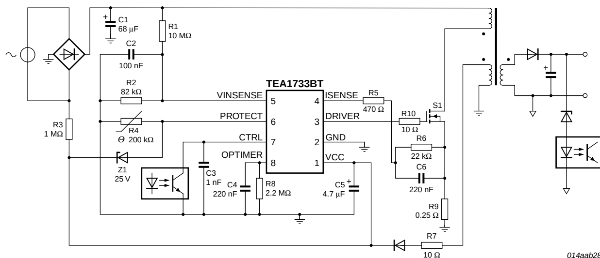
Fig 10. Typical application
