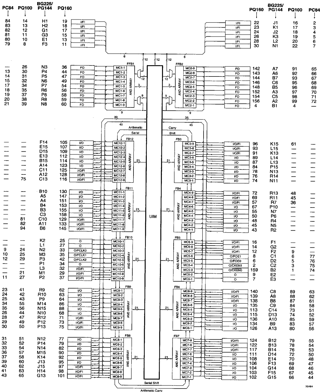
Figure 2: XC73108 Architecture
