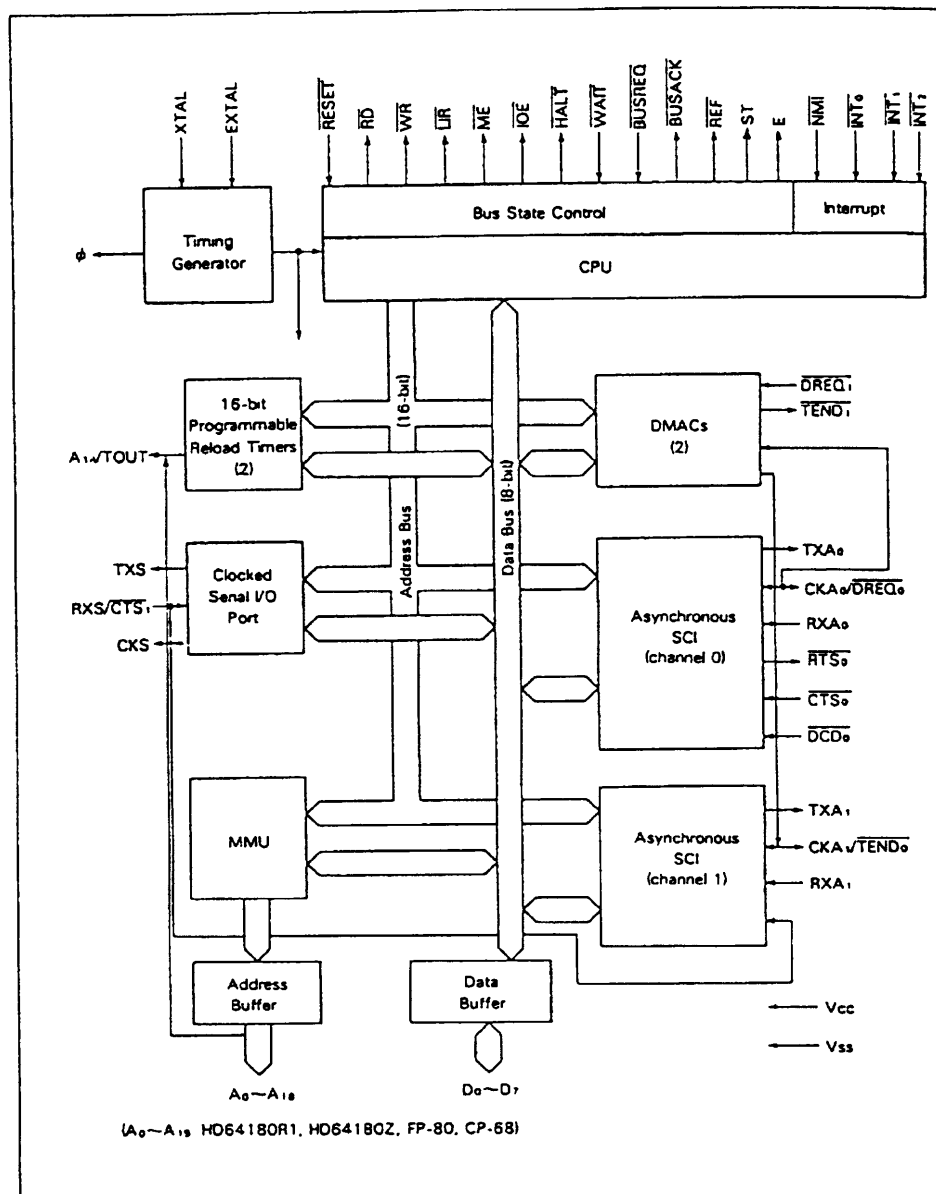
Figure 1.1.1 Block Diagram
