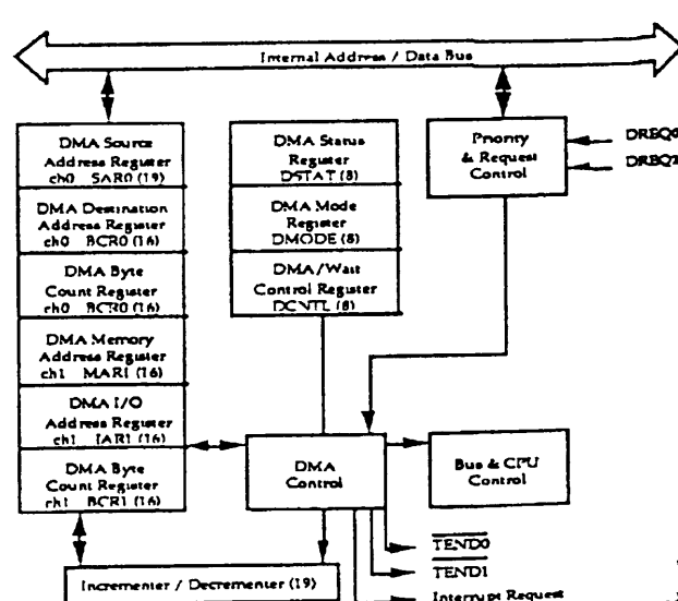
DMAC Block Diagram
