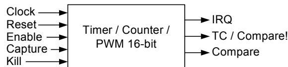
Figure 7-19. Timer/Counter/PWM
