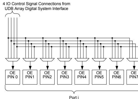
Figure 7-17. I/O Pin Output Enable Connectivity
