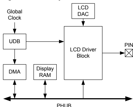
Figure 8-7. LCD System
