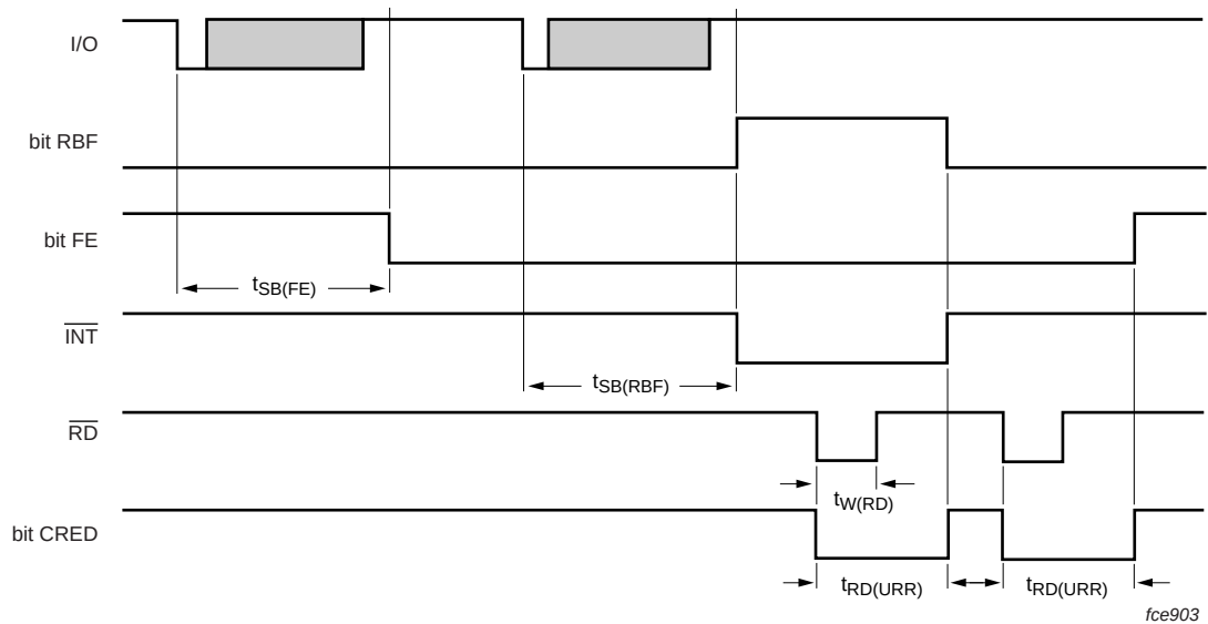
Fig 13. Minimum time between two read operations in register URR - multiplexed mode TDA8007BHL/C3
