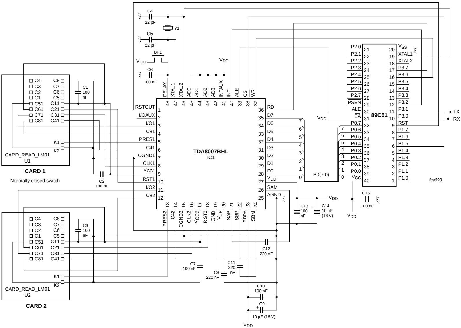
Fig 21. TDA8007BHL/C3 application
