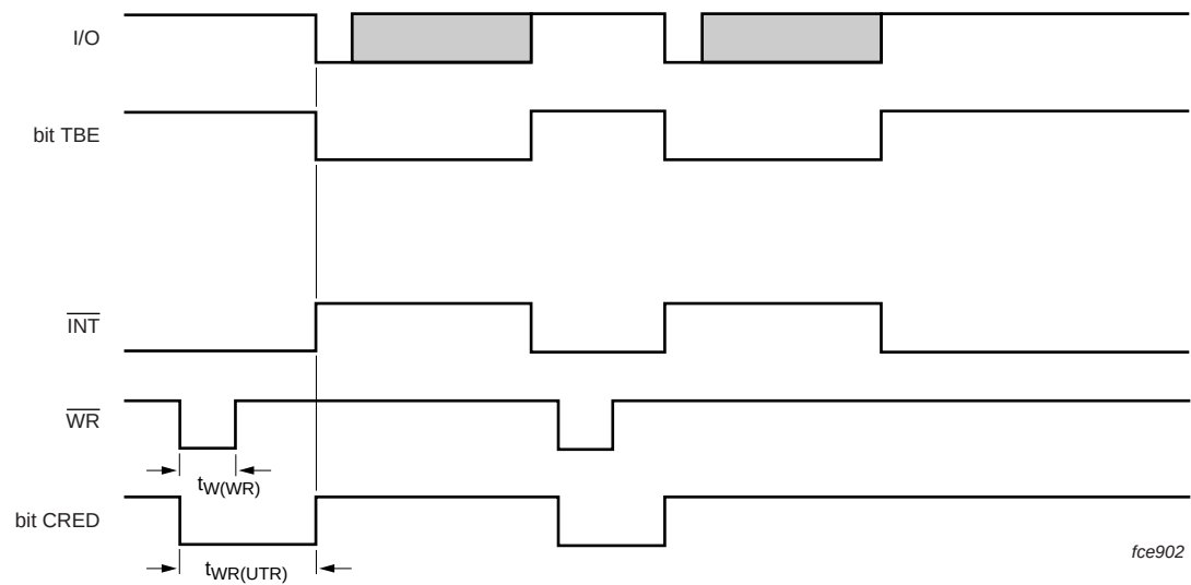
Fig 14. Minimum time between two write operations in register UTR - multiplexed mode TDA8007BHL/C3
