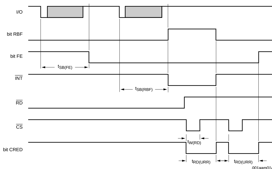
Fig 10. Minimum time between two read operations in register URR - non-multiplexed bus
