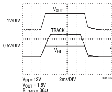
Output Tracking
