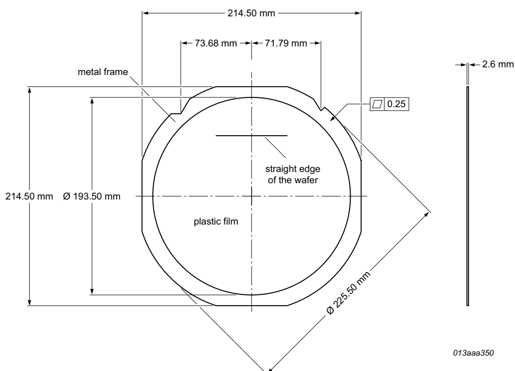
Fig 31. Film Frame Carrier (FFC) for 6 inch wafer (PCF8564AU/10AB/1)
