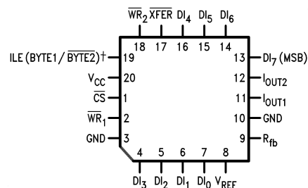
Figure 2. PLCC Package
