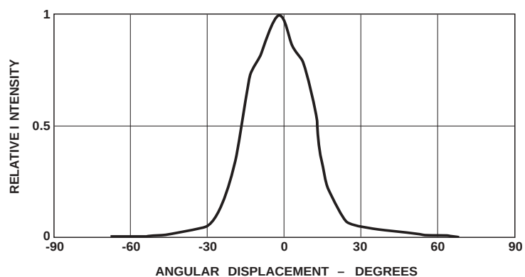
Figure 8. Spatial radiation pattern – 30 degree lamps.
