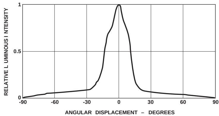
Figure 7. Spatial radiation pattern – 23 degree lamps.
