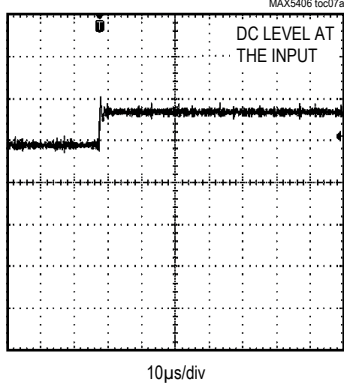
WIPER SWITCHING TRANSIENT
