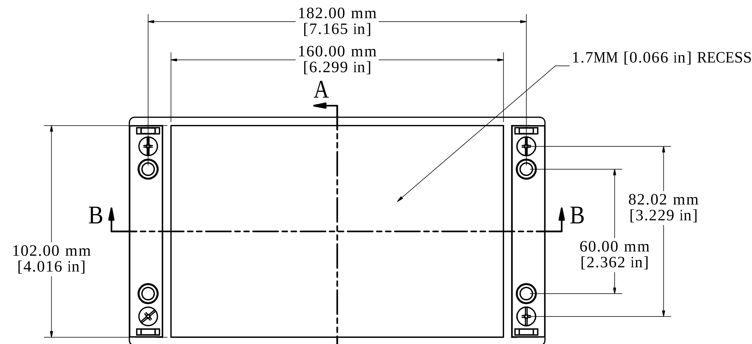
ASSEMBLY - TOP VIEW
