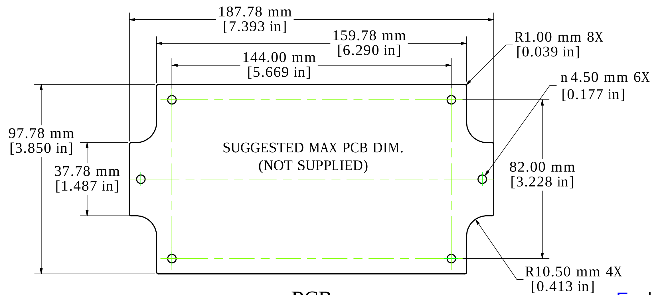
PCB
