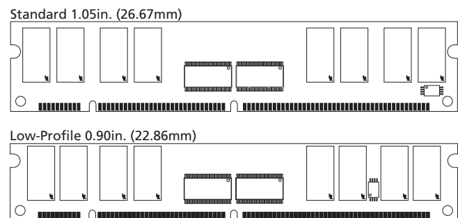
Figure 1: 168-Pin DIMM (MO-161)
