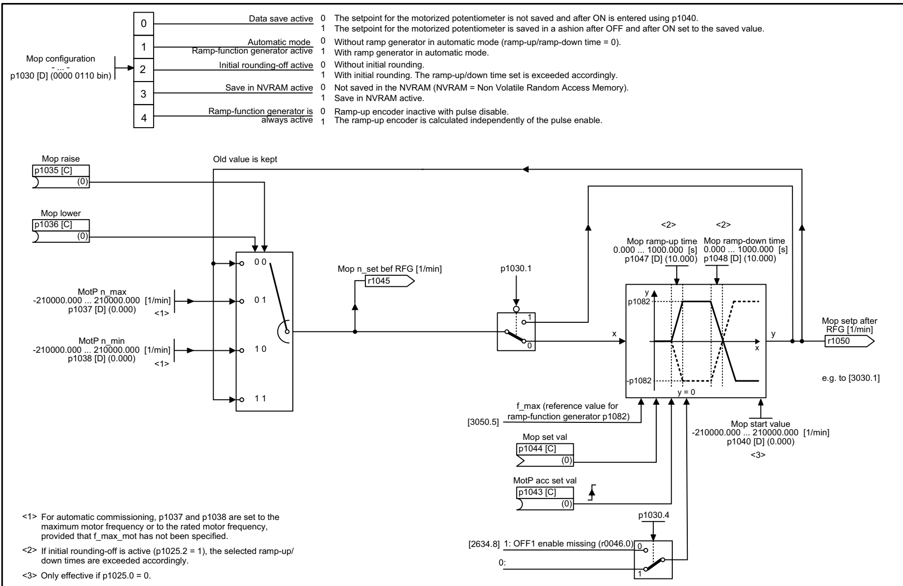
Fig. 2-64 3020 – Motorized potentiometer
