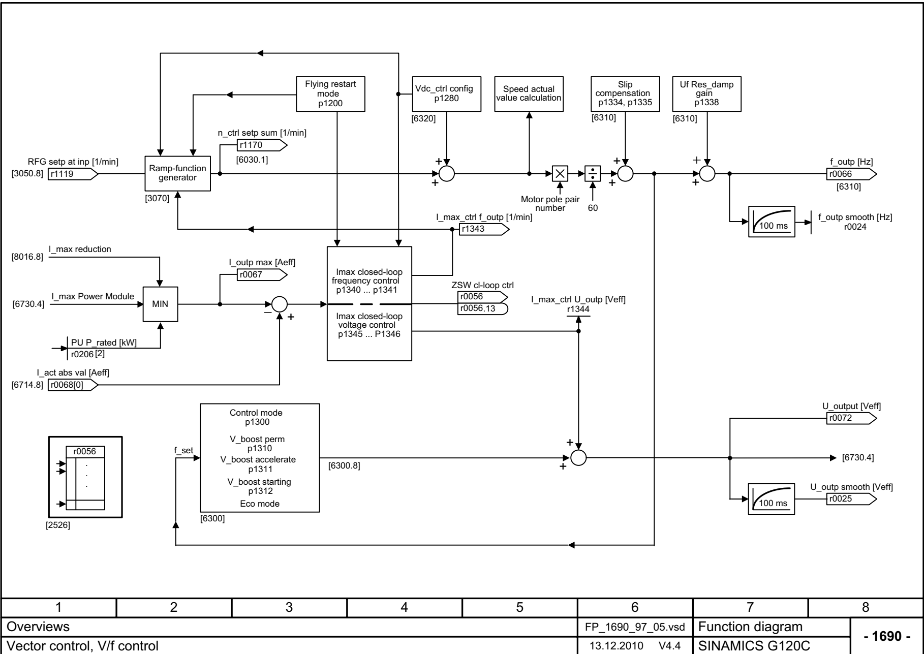
Fig. 2-8 1690 – Vector control, V/f control
