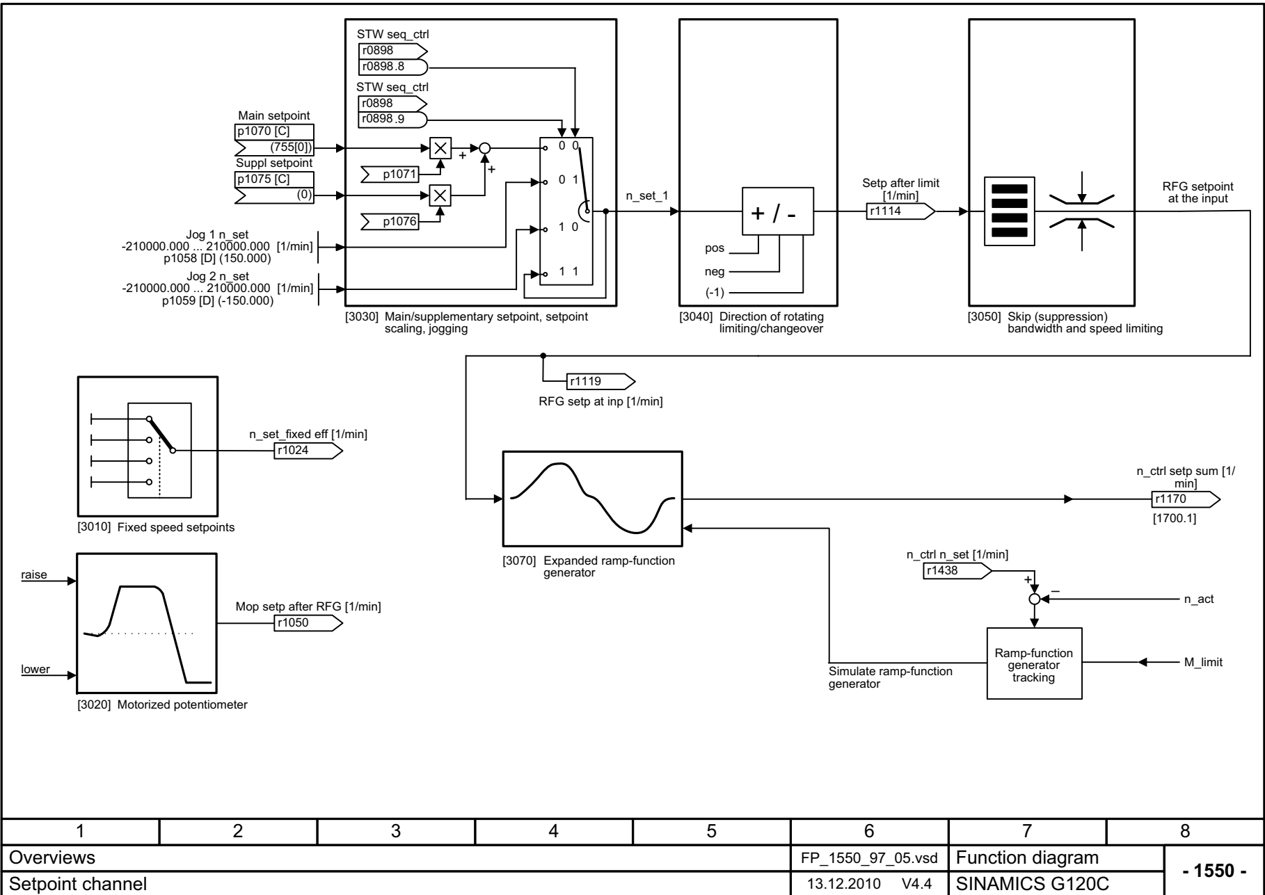
Fig. 2-7 1550 – Setpoint channel
