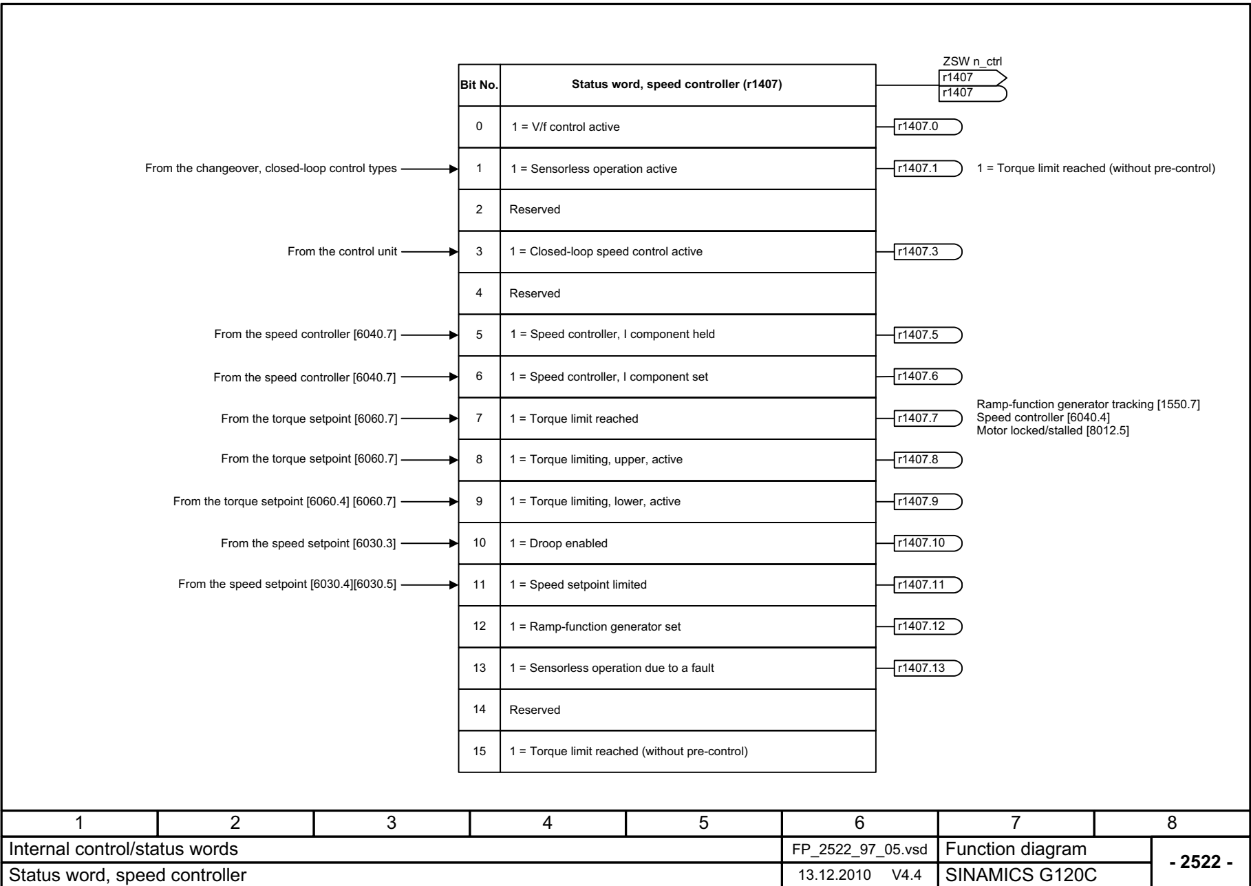
Fig. 2-47 2522 – Status word, speed controller
