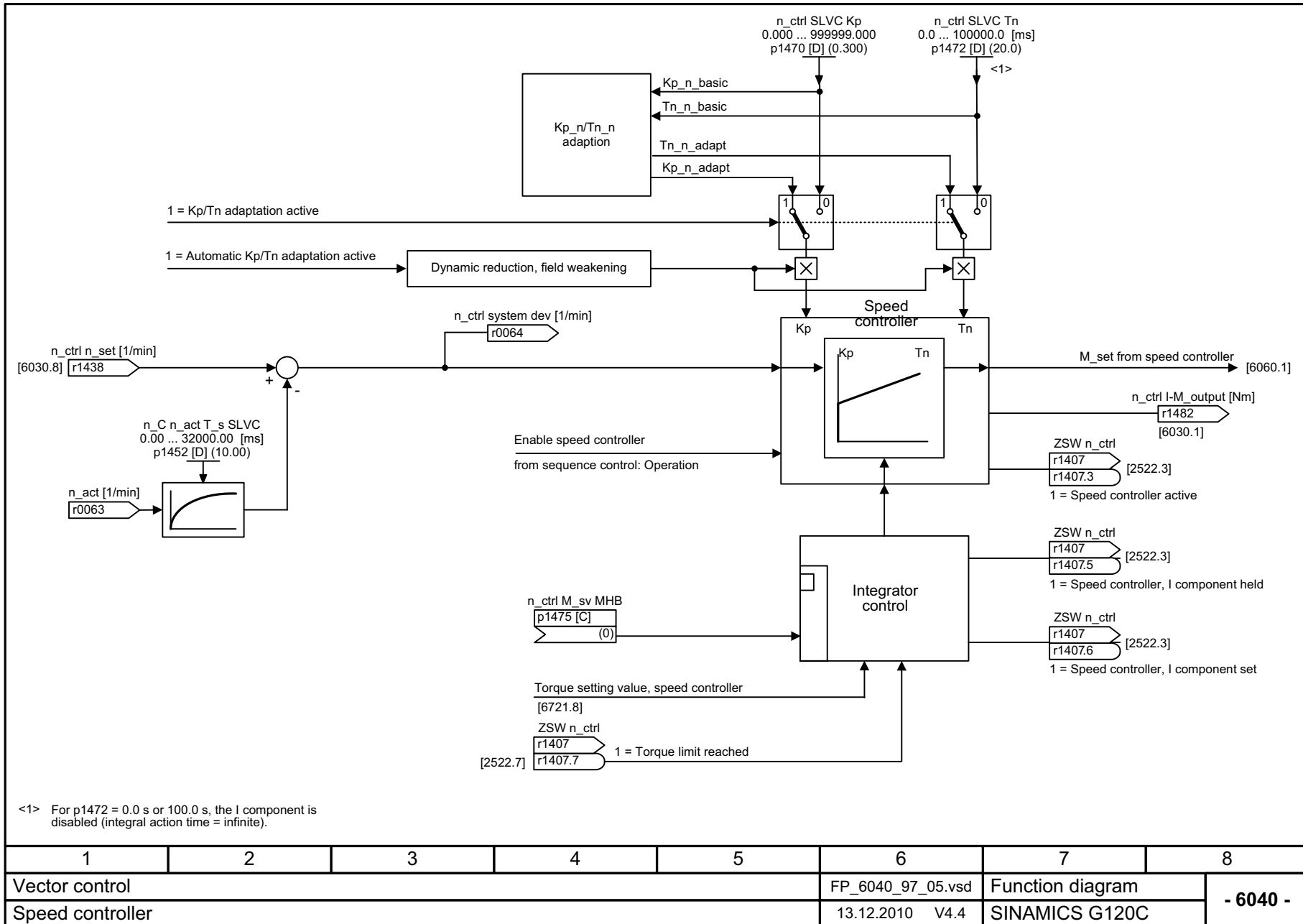
Fig. 2-73 6040 – Speed controller
