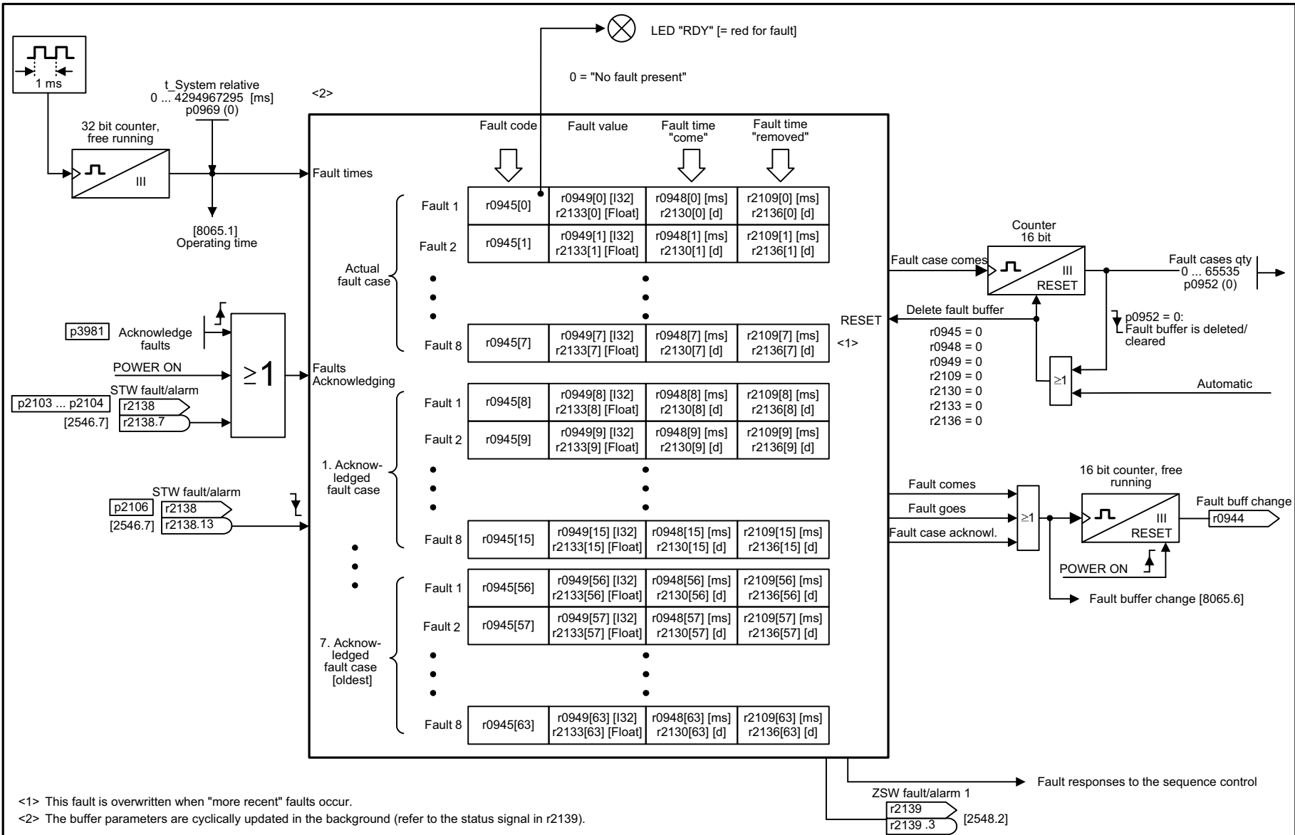
Fig. 2-100 8060 – Fault buffer
