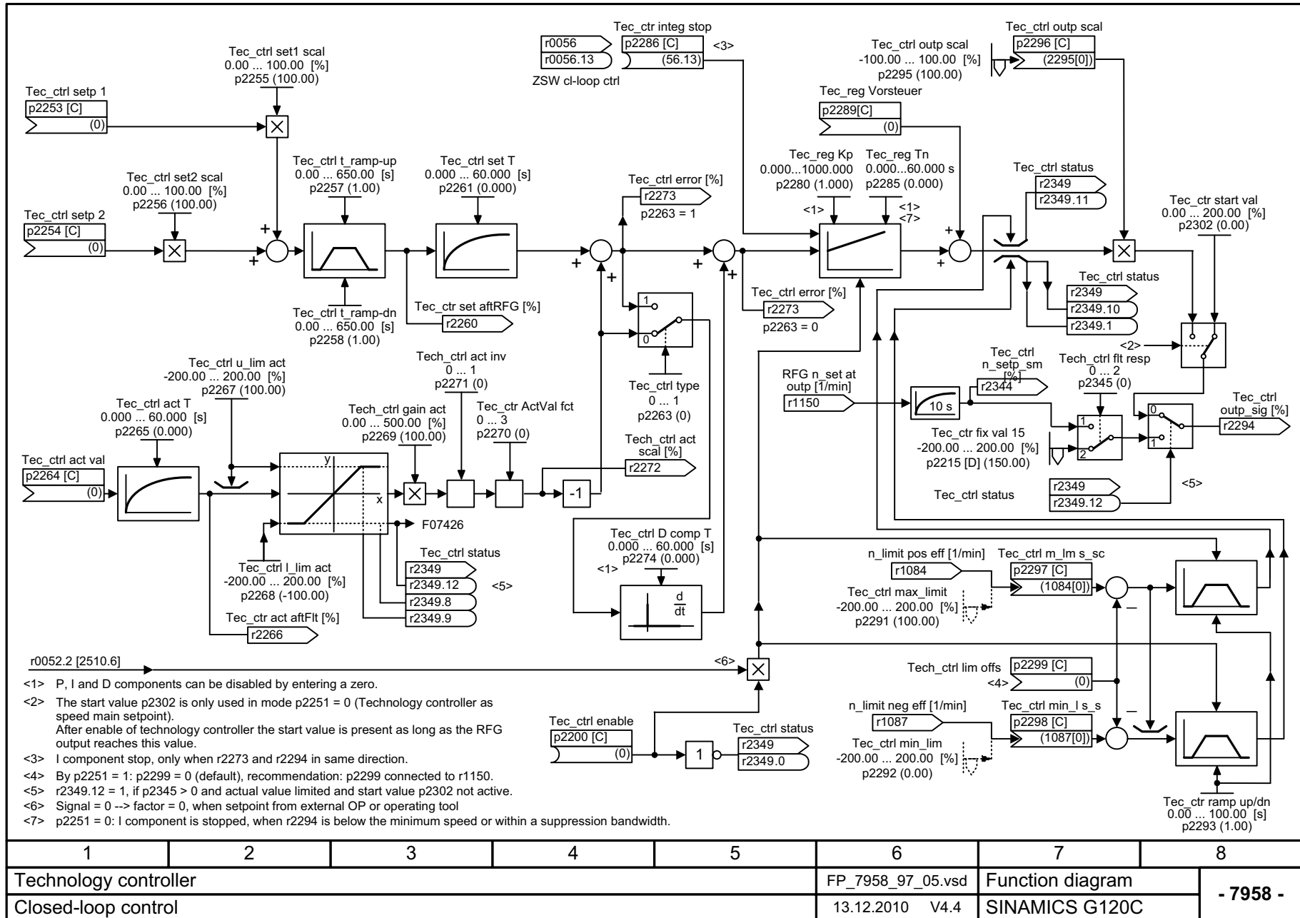
Fig. 2-91 7958 – Closed-loop control
