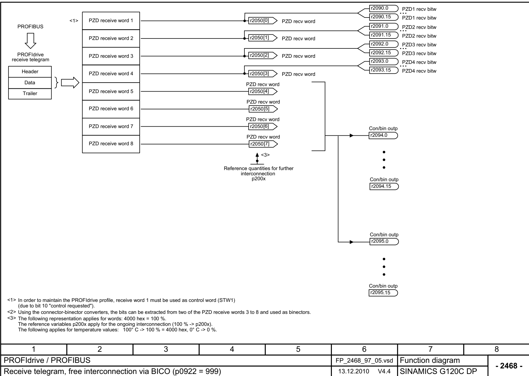
Fig. 2-32 2468 – Receive telegram, free interconnection via BICO (p0922 = 999)
