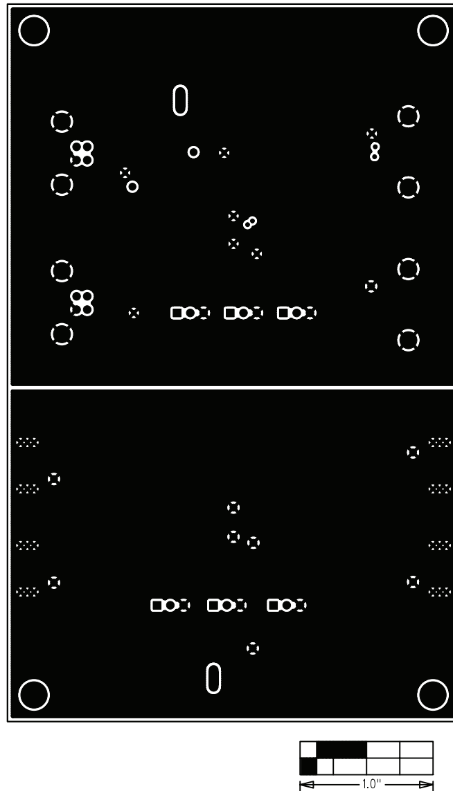
Figure 4. MAX4989 EV Kit PCB Layout—Layer 2
