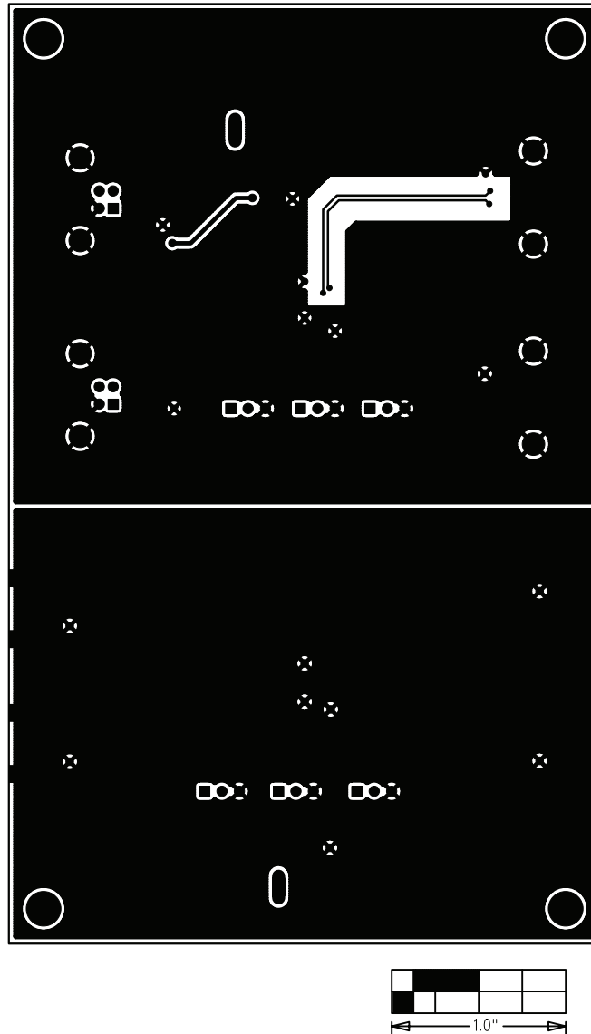
Figure 6. MAX4989 EV Kit PCB Layout—Solder Side
