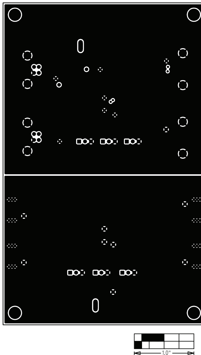
Figure 5. MAX4989 EV Kit PCB Layout—Layer 3
