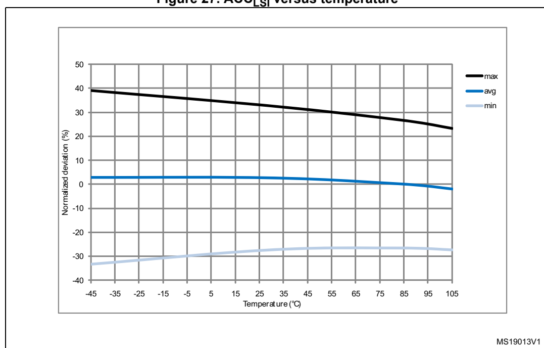
Figure 27. \text{ACC}_{\text{LSI}} versus temperature
