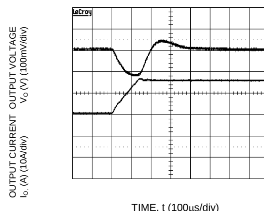
Figure 18. Transient Response to Dynamic Load Change from 50% to 75 % of full load current.
