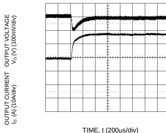
Figure 42. Transient Response to Dynamic Load Change from 50% to 75 % of full load current.
