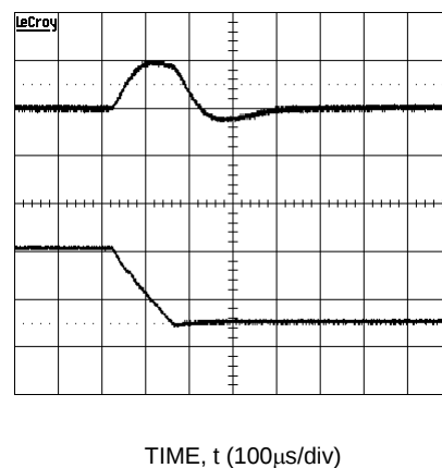
Figure 17. Transient Response to Dynamic Load Change from 50% to 25% of full load current.
