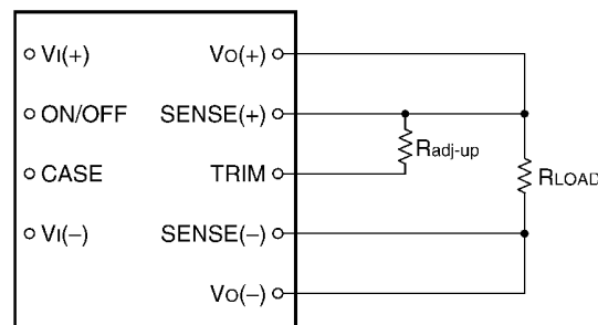
Figure 49. Circuit Configuration to Increase Output Voltage.
