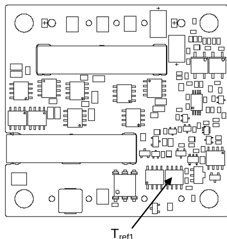
Figure 50. T_{ref} Temperature Measurement Location for V_o = 12V .
