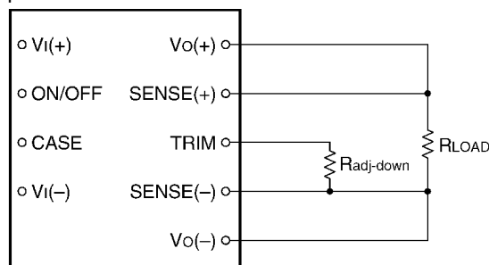
Figure 48. Circuit Configuration to Decrease Output Voltage.
