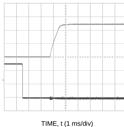
Figure 4. Typical Start-Up Characteristics from Remote ON/OFF.
