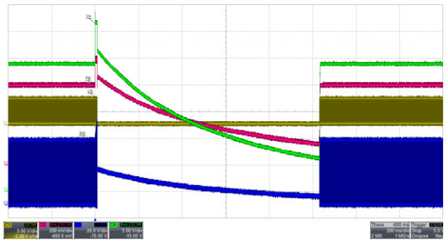
Figure 33. OVP2 Release at V_{FB} \leq 100\% V_{REF}
