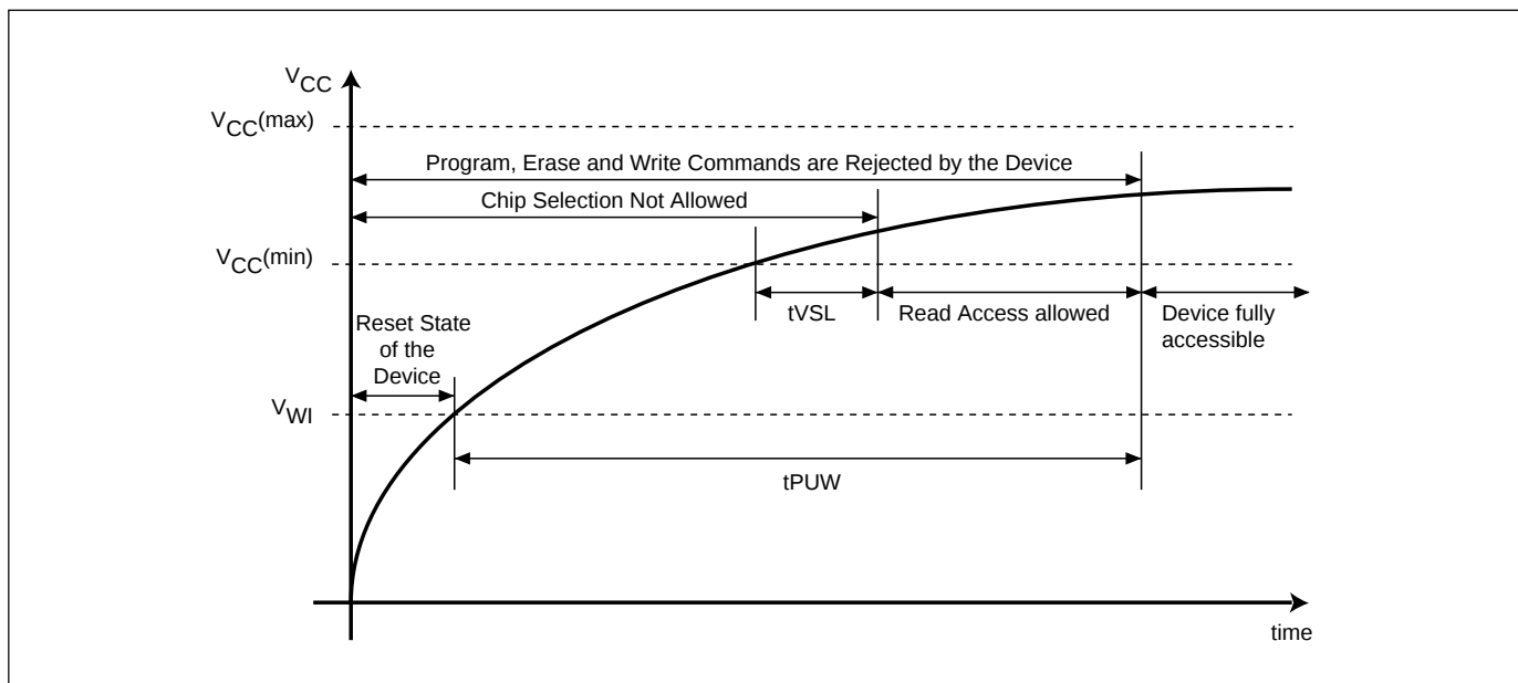
Figure 26. Power-up Timing
