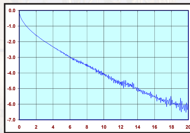
PN: CCSMA-MM-SS402-120 INSERTION LOSS (S12)
