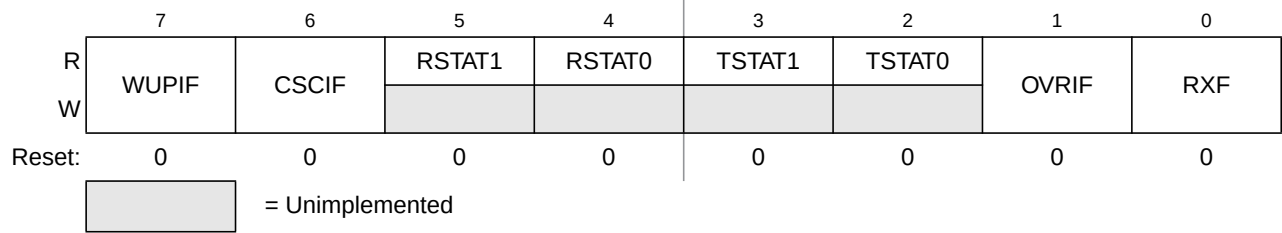
Figure 8-8. MSCAN Receiver Flag Register (CANRFLG)
