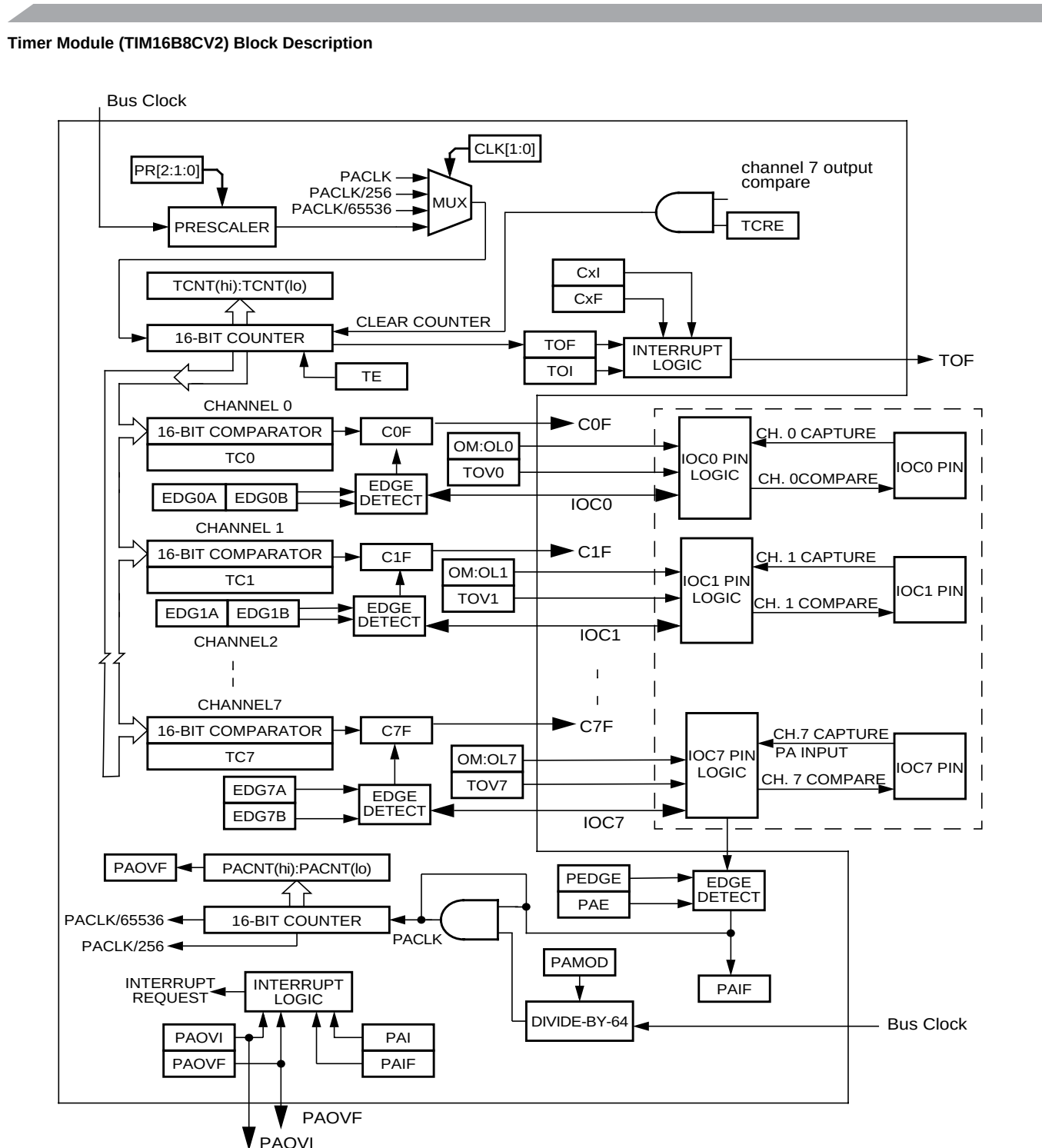
Figure 14-30. Detailed Timer Block Diagram
