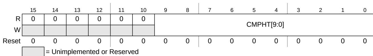
Figure 9-13. ATD Compare Higher Than Register (ATDCMPHT)
