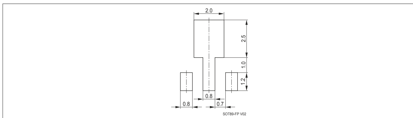
Figure 25 Package Footprint (dimension in mm)
