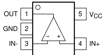
TL391B-Q1 DBV Package 5-Pin SOT-23 Top View
