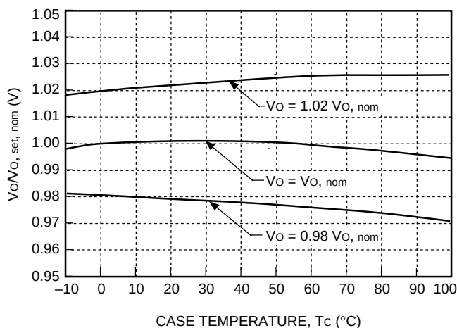
Figure 2. MA010-Series Typical Output Voltage Variation Over Operating Case Temperature
