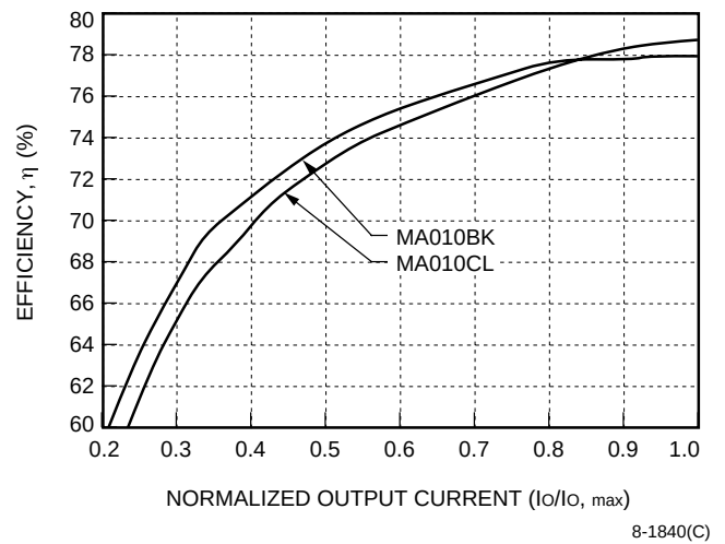
Figure 8. MA010BK, CL Typical Converter Efficiency as a Function of Output Current with V_I = 12 V and T_A = 25 °C
