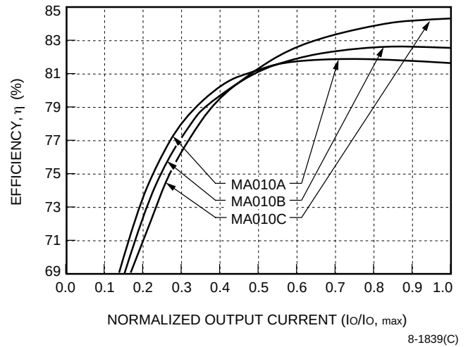
Figure 7. MA010A, B, C Typical Converter Efficiency as a Function of Output Current with V_I = 12 V and T_A = 25 °C
