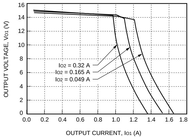
Figure 6. MA010CL Typical Output Characteristics with V_I = 12 V, T_A = 25 °C
